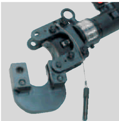
S-40B (Head opened)
