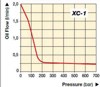
OIL FLOW vs. PRESSURE
